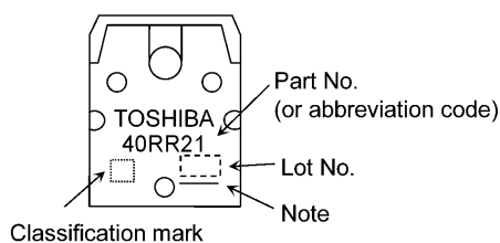
Fig. 7.1 Marking
