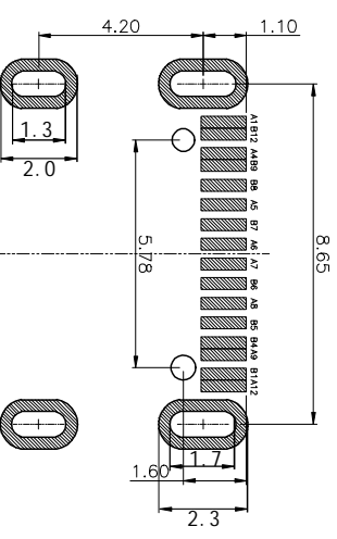
PCB LAYOUT(Recommend) (General Tolerance:±0.05)
